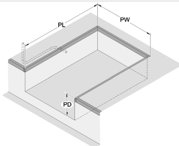
pit drawing 5143.0186
