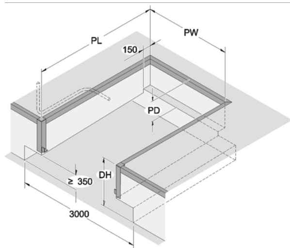
pit drawing 5143.0180
