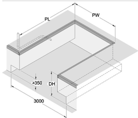
pit drawing 5143.0177
