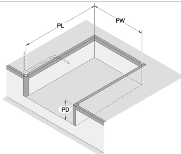
pit drawing 5143.0185
